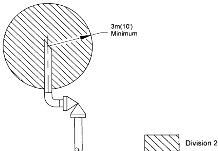
Figure 18—Relief Valve in a Nonenclosed Adequately Ventilated Area
