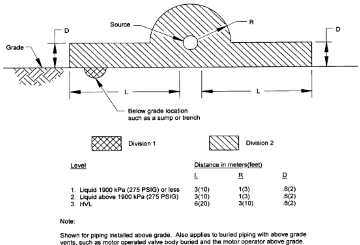
Figure 96—Outdoors—Piping With Valves, Screwed Fittings, Flanges or Similar Accessories Handling Flammable Liquids or Highly Volatile Liquids. Also Covers Sampling Systems, Instrumentation and Instrument-Sized Pumps
