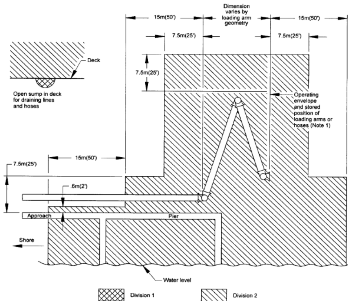
Figure 19—Marine Terminal Handling Flammable Liquids
